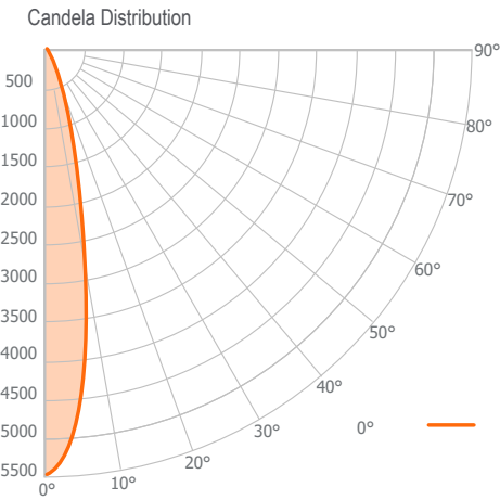
3" Pendant with Wide Shade
