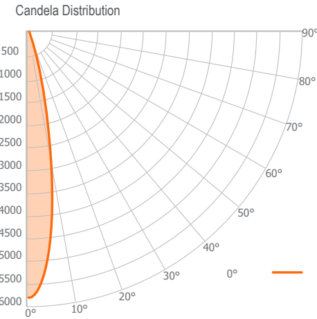
3" Pendant with Narrow Shade
